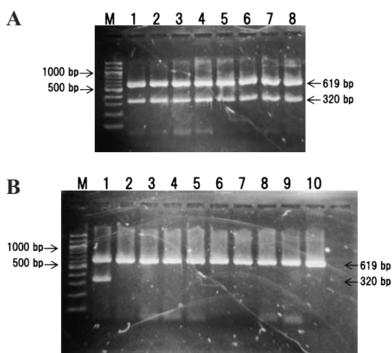
Fig. 1. A: lane 1: ipaH/ial positive control strain ( S. dysenteriae 93SHL), lane 2: 02SHL5, lane 3: 02SHL6, lane 4: 03SHL14, lane 5: 04SHL19, lane 6: 04SHL22, lane 7: 04SHL23, lane 8: 02SHL25, lane M: molecular marker (100 bp ladder). B: lane 1: ipaH/ial positive control, lane 2: 02SHL1, lane 3: 02SHL2, lane 4: 02SHL3, lane 5: 02SHL4, lane 6: 02SHL7, lane 7: 03SHL8, lane 8: 03SHL15, lane 9: 03SHL16, lane 10: 04SHL17, lane M: molecular marker (100 bp ladder).
